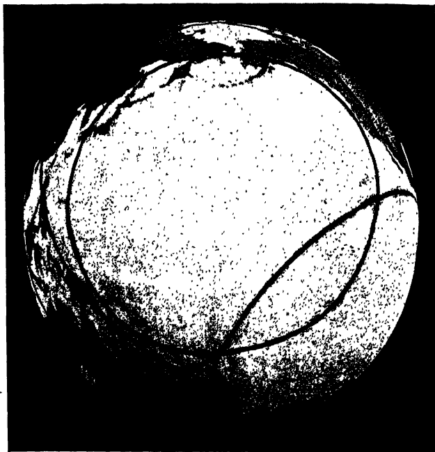
FIG. 38.—North Pacific view of the globe, showing the relations of the abyssal basin to North America, Asia, and Australasia, to the Alaska-Siberian bridge, and to the South Pacific.
