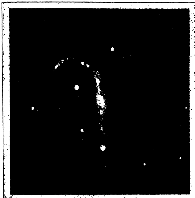
FIG. 18a.—A spiral nebula in which the two arms are especially distinct, HI 55 Pegasi.
