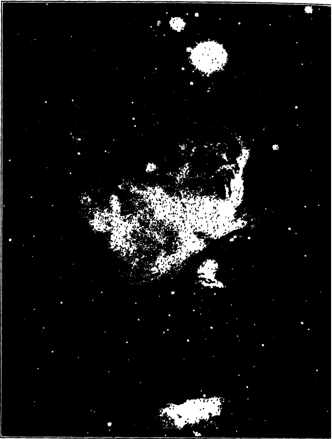
FIG. 3.—The Great Nebula in Orion and the Fish-Mouth Nebula. Photographed at the Yerkes Observatory.
