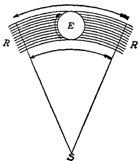
FIG. 4.—RR represents a ring of gas moving as a unit and hence the outer portion the faster. If converted into a spheroid, E , centrally located, the rotation is forward, as shown by the arrow.
