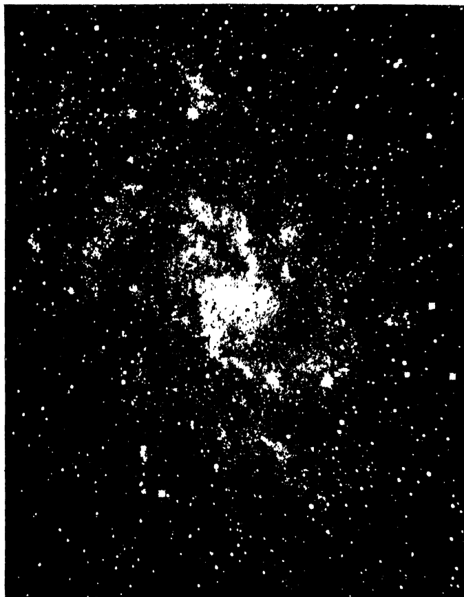
FIG. 19.—A strongly deployed giant nebula, M 33, in Triangulum. Photographed at the Yerkes Observatory.
