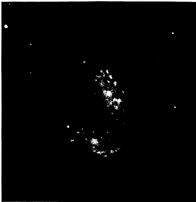
FIG. 25.—A double spiral nebula, N.G.C. 4567 and 4568. Photographed at the Mount Wilson Solar Observatory.
