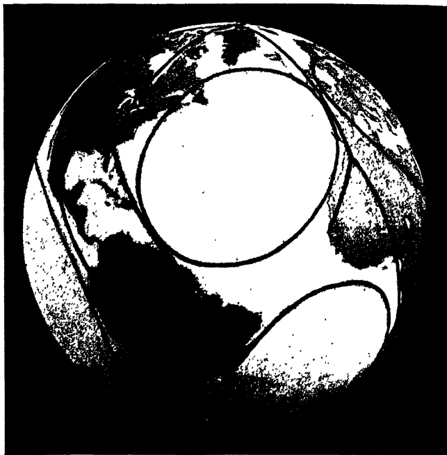
FIG. 35.—North Atlantic view of the globe, showing the relations of the coalescent ocean basins to the yield-tracts lying west of them, particularly those of the West Indies.
