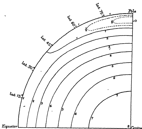
FIG. 26.—Diagram showing curves of equal stress-difference due to the weight of second harmonic inequalities or to tide-generating force. (Darwin.)
