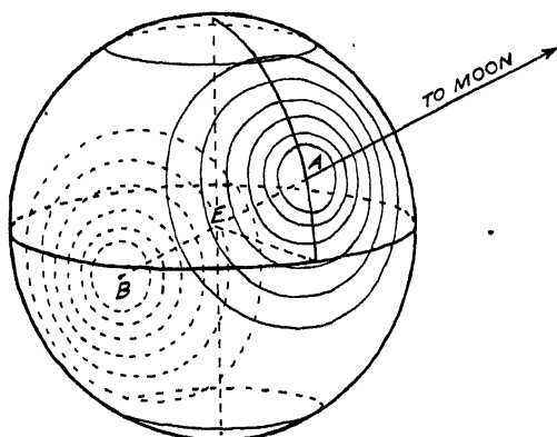
FIG. 13.—Diagram showing the tidal cones, A and B , pointing to and from the moon. Prepared by F. R. Moulton.
