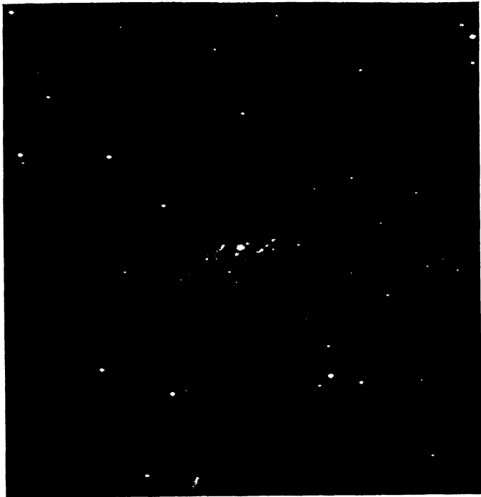
FIG. 15.—Spiral nebula HV 2 Virginis. Photographed at the Lick Observatory.
