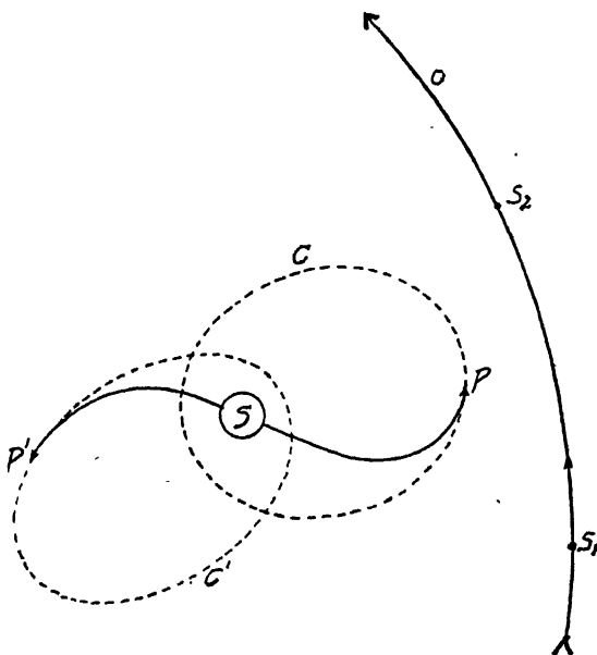
FIG. 18.—Diagram showing an assigned mode of developing orbits (Moulton).
