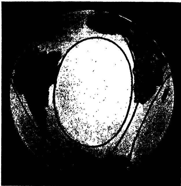
FIG. 31.—South Atlantic view of the globe, showing also the South American and South African bifurcations and angulations of the main structure lines and yield-tracts, indicated by the straight lines which outline the quadrilaterals inclosing the oceans.
