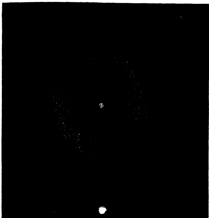
FIG. 2.—The ring nebula in the constellation Lyra. Photographed at the Lick Observatory.
