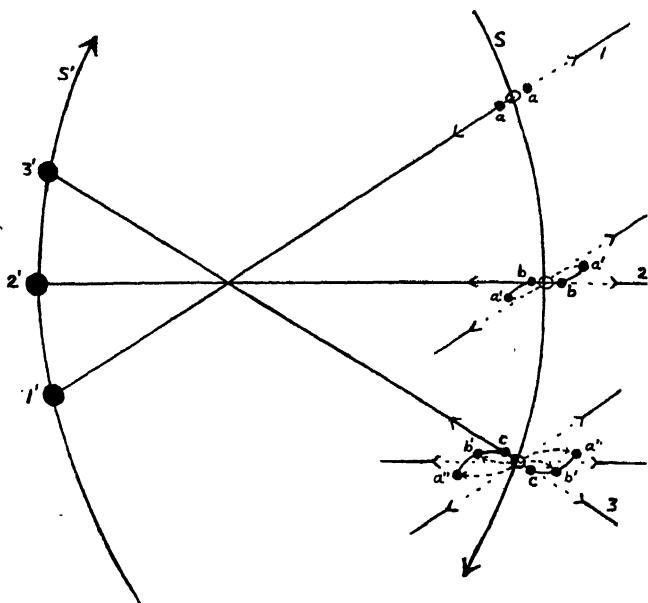
FIG. 17.—Diagram showing one of the assigned modes of development of a spiral nebula.
