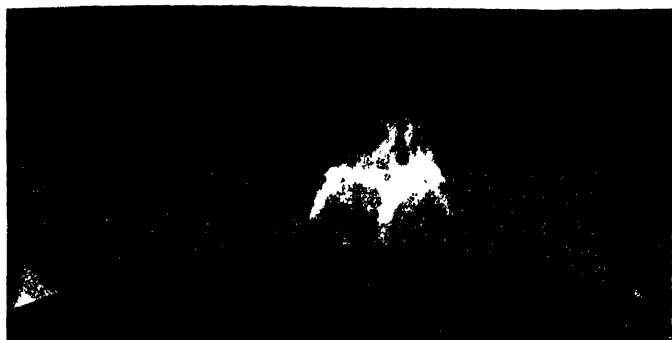
FIG. 10.—Eruptive prominence of the sun photographed at Yerkes Observatory March 25, 1910, at 4h 14.7m.
