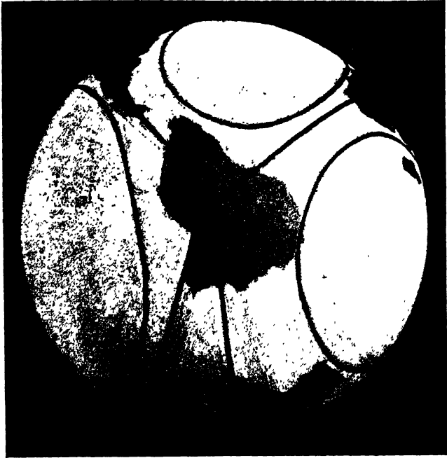
FIG. 30.—South polar view of the globe showing the relations of the southern points of South America, Africa, and Australia to Antarctica and the South Pole, and the tripartite division of the south polar region. The radiant lines merely suggest the approximate positions of the yield-tracts, which of course take on natural flexures. The ovals suggest the somewhat circular configuration of the oceans.
