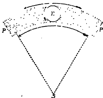
FIG. 5.— PP represents a belt of planetesimals revolving concentrically about the center, S . If these collect about the central point of the belt into a spheroid, E , by the enlargement of the inner orbits or the reduction of the outer ones, the concentric arrangement remaining, the rotation will be retrograde, as shown by the arrow.
