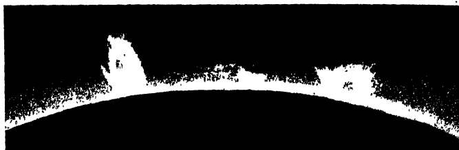
FIG. 8.—Solar prominences illustrating the eruptive state of the sun. Photograph taken during eclipse May 28, 1900, Yerkes Observatory.
