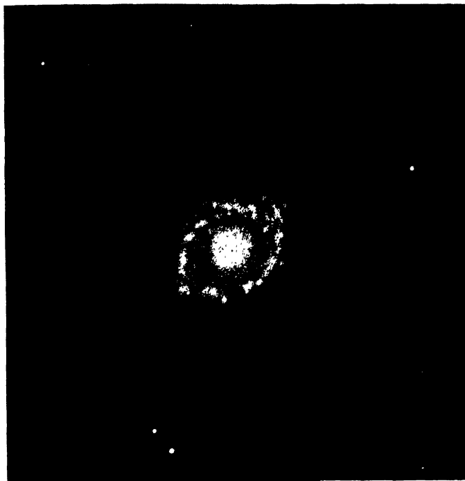
FIG. 20.—A spiral nebula with large knots wrapped about a large center. M 94 (N.G.C. 4736) Canum Venaticorum. Photographed at the Mount Wilson Solar Observatory.
