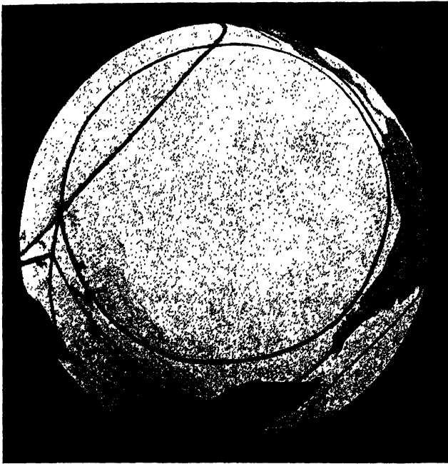
FIG. 37.—South Pacific view of the globe and the adjacent yield-tracts on the east, south, and west, and its coalescence with the North Pacific, indicated by the overlapping of the circles, which define the fundamental circularity of the oceans.
