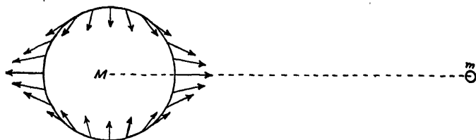
FIG. 12.—Diagram of tidal forces showing lifting forces in due proportions and directions to and from the moon and the girdle of compressive forces at right angles to these. Note that the direct compression is half that of direct lifting. Prepared by F. R. Moulton.
